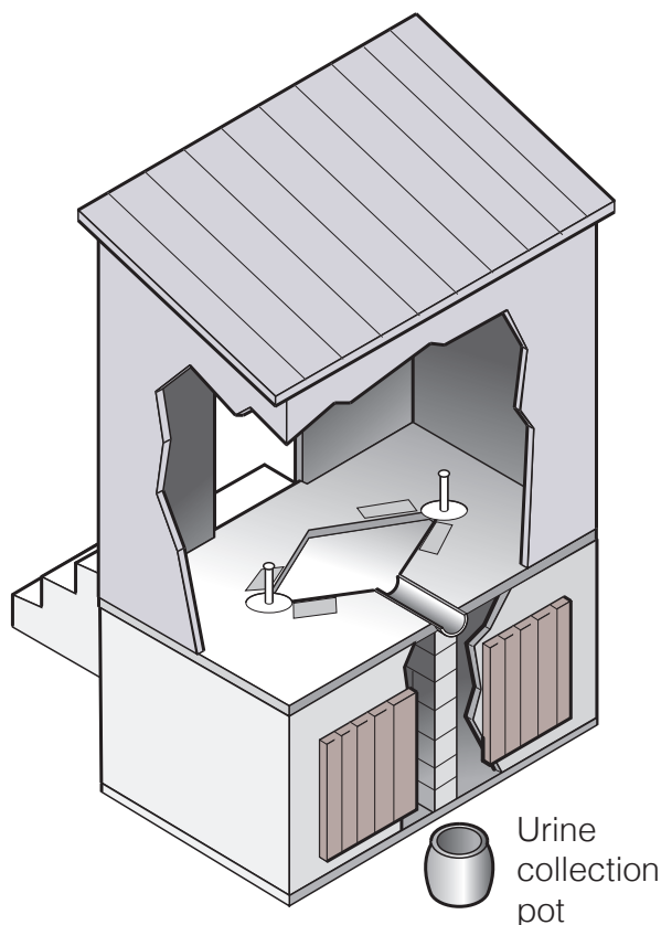
Figure 8. Urine diversion toilets require specific slab designs
