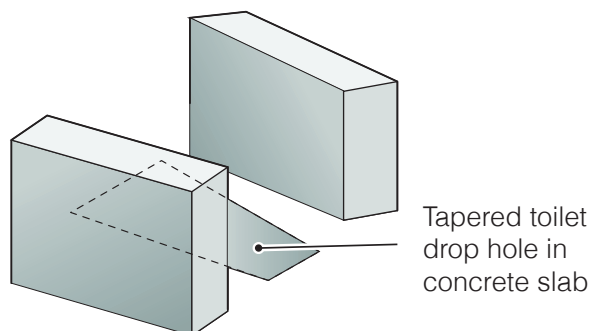
Figure 22. Concrete blocks can form a simple pedestal
