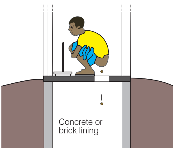
Figure 25. Well-supported slabs can be smaller
