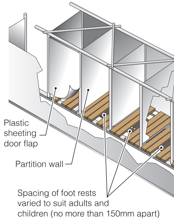
Figure 28. Temporary wooden slabs may only be acceptable in the initial stages of an emergency
