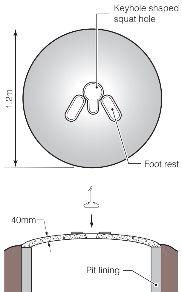
Figure 17. A domed slab
