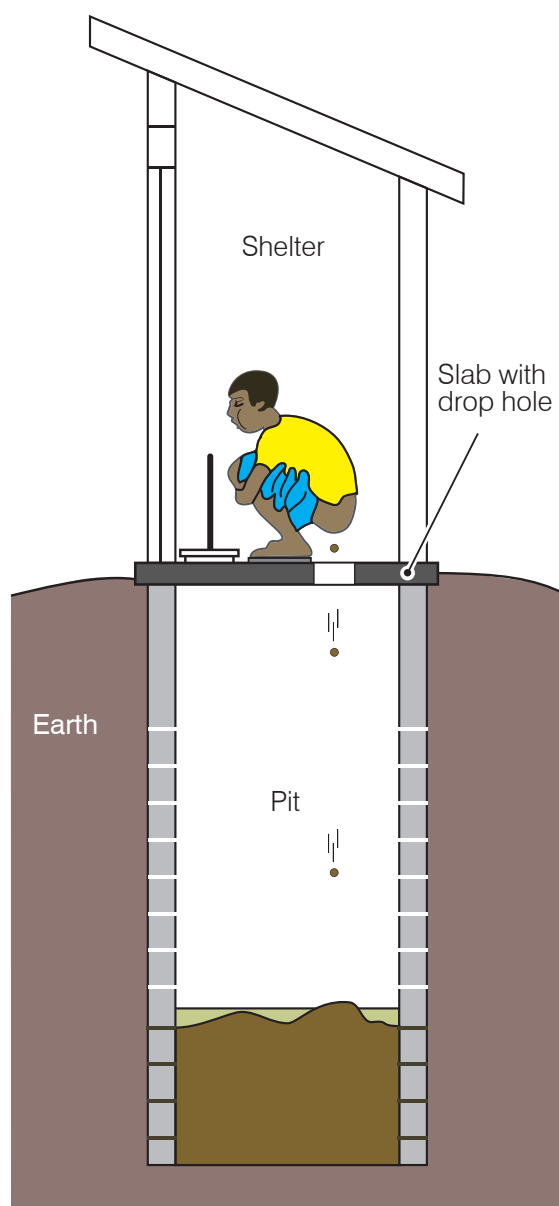
Figure 1. A simple pit latrine
