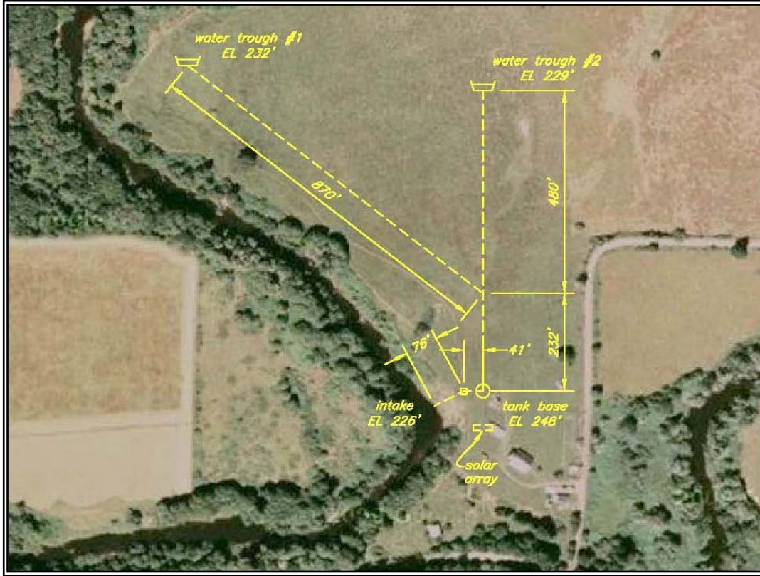
Figure 12 – A plan of an example watering system with a storage tank and PV array.
