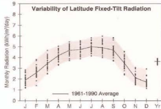
Solar Radiation for Flat-Plate Collectors Facing South at a Fixed Tilt (kWh/m 2 /day), Uncertainty ±9%
