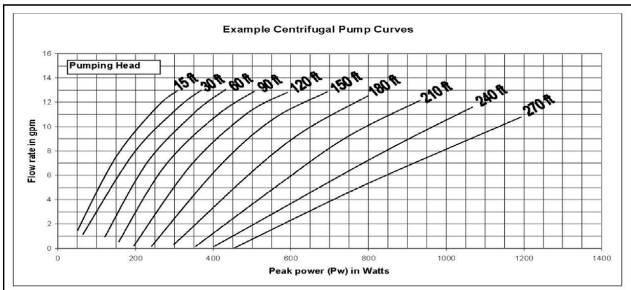
Figure 11 – Example solar-powered pump performance curves for a centrifugal pump.
