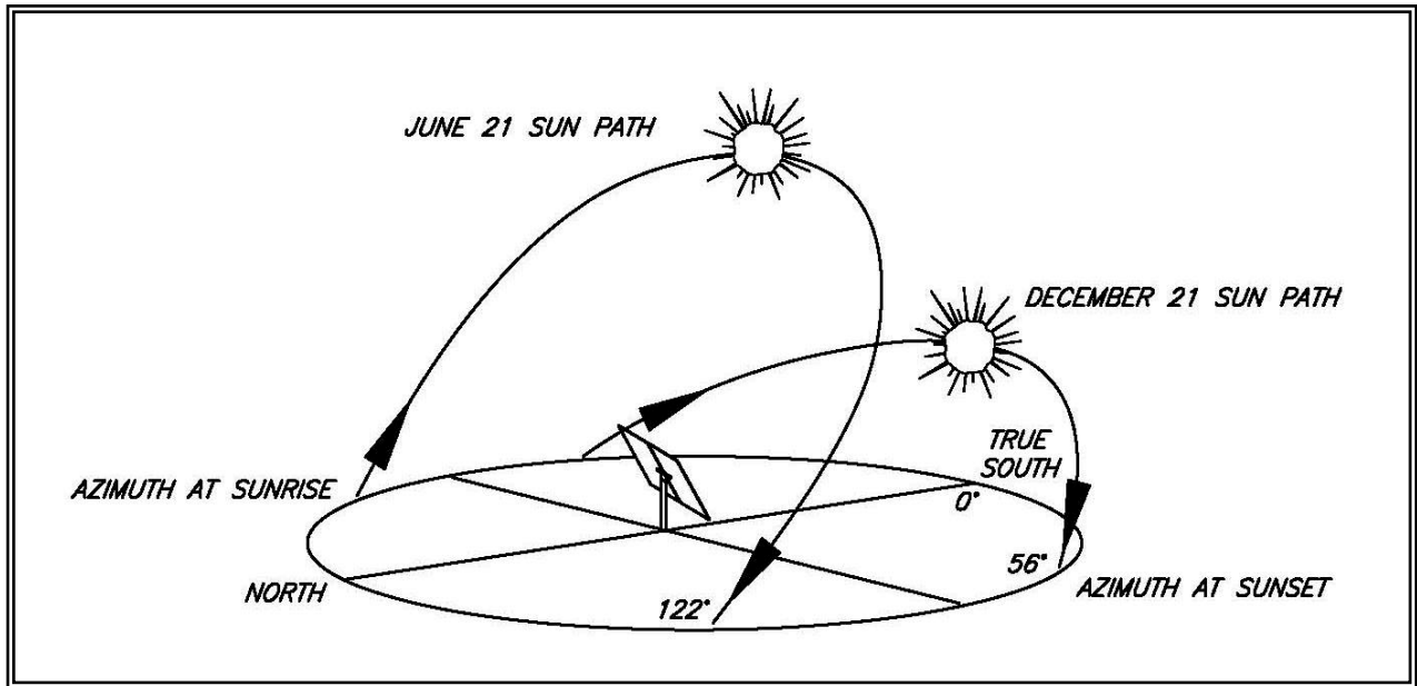
Figure 4 – Example summer and winter sun elevation and angle. (Source: “Renewable Energy Primer-Solar.”)
