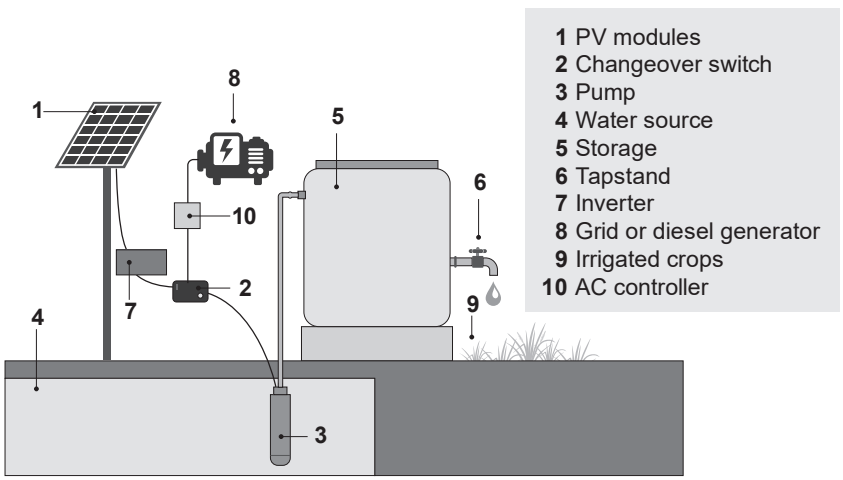
Figure 3.3 Hybrid installation
