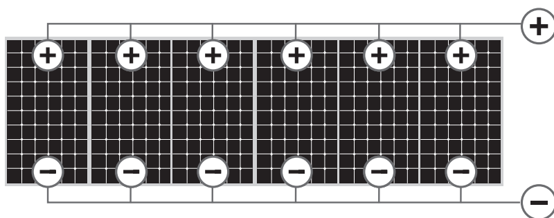
Figure 5.2 Parallel connection
