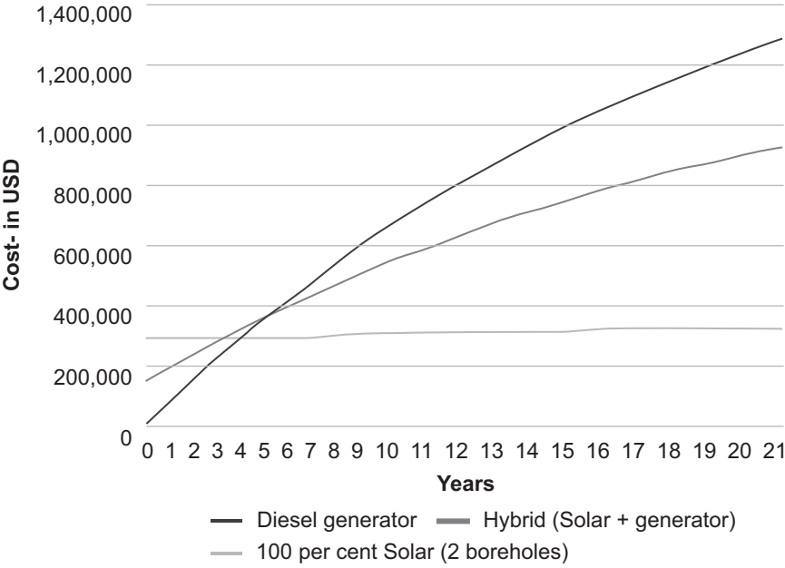
Figure 9.3 LCCA of stand-alone generator vs hybrid vs solar at Nyarugusu, Tanzania
