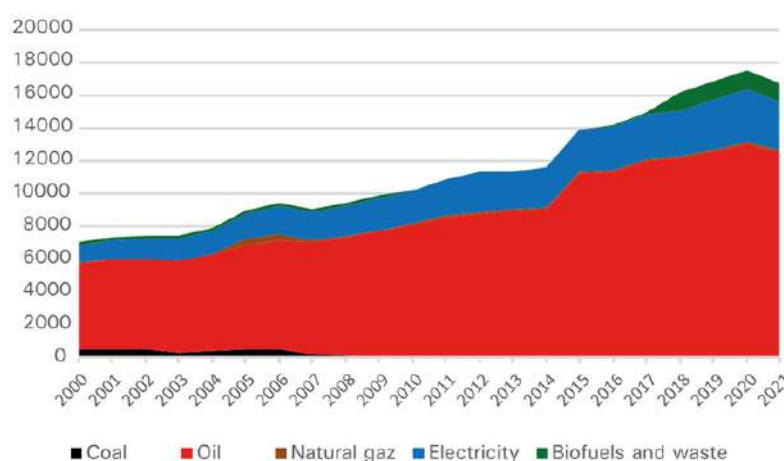
Figure 30: Morocco Total Final Consumption (ktOE) 19 ( AFREC, 2022 )
