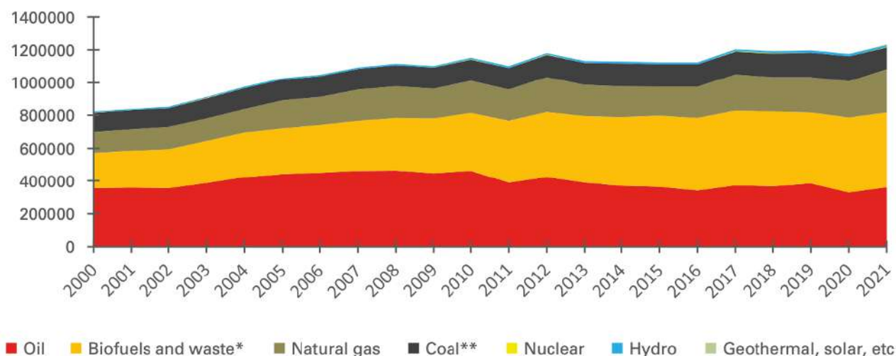
Figure 10: Total Primary Energy Supply (TPES) from 2000 to 2021 by fuel (ktoe) ( AFREC, 2023 ) * Includes firewood, charcoal, biogas, agro residues, waste, and others biomass ** Includes steam coal, coking coal, lignite and recovered coal.
