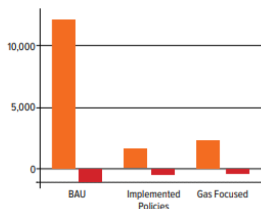
Figure 25: Additional costs related to premature deaths compared to the capex in the NZ scenario (mil US$) (MOEP 2024)
