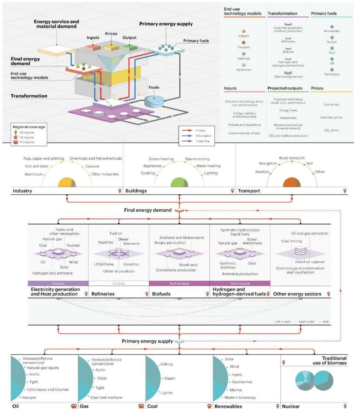
Figure 7: Detailed view of IEA's Global Energy and Climate (GEC) model (IEA, 2023).
