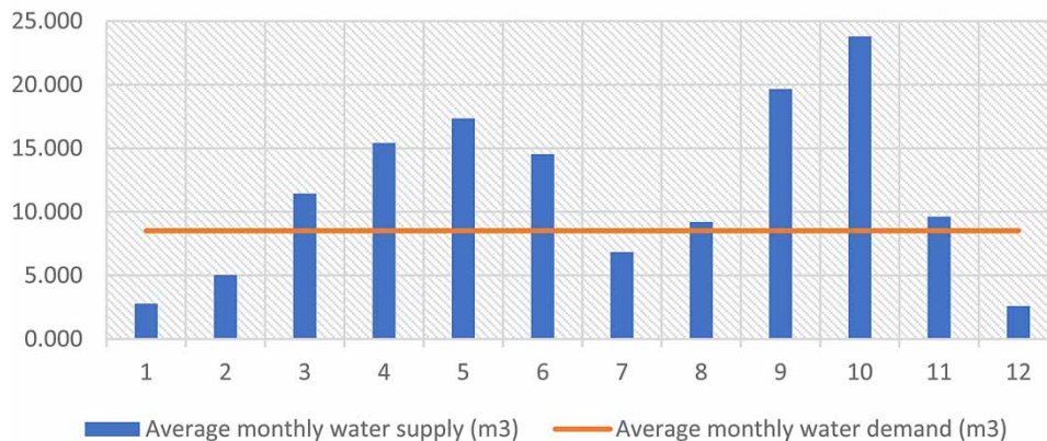
Figure 8 | Average monthly rainwater supply and population's demand.
