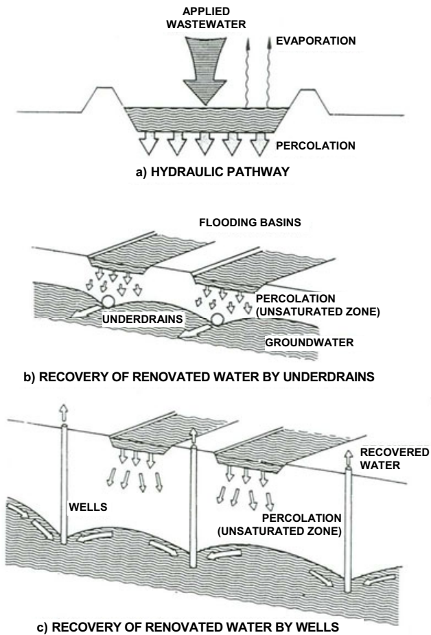
Figure 8.3 Rapid infiltrations (U.S.EPA 1981)
