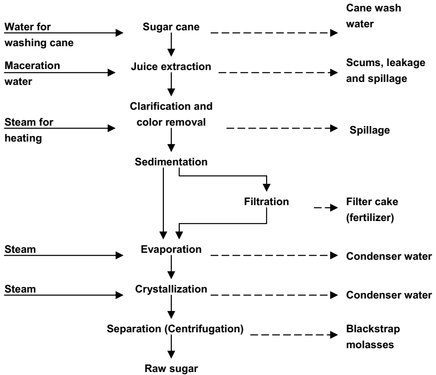
Figure 2.6 Diagrammatic flow sheet of the process of raw sugar manufacture (adapted from Meade and Chen 1977)
