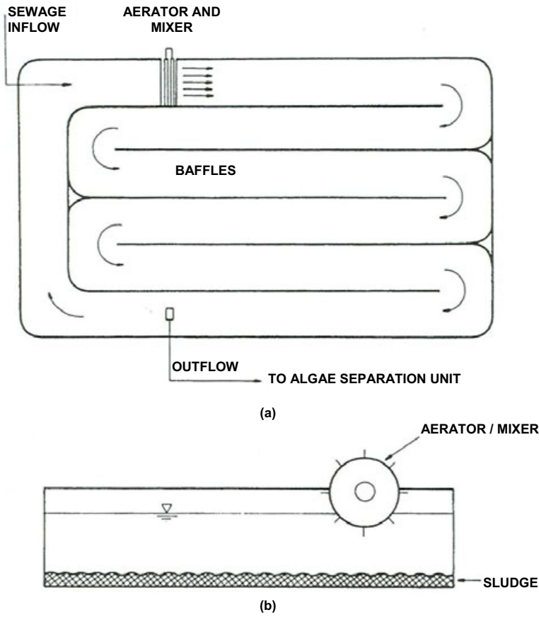
Figure 5.5 High-rate algal pond: (a) schematic plan, (b) schematic cross-section
