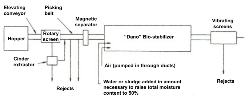
Figure 3.17 Typical DANO plant (after Flintoff and Millard 1969)
