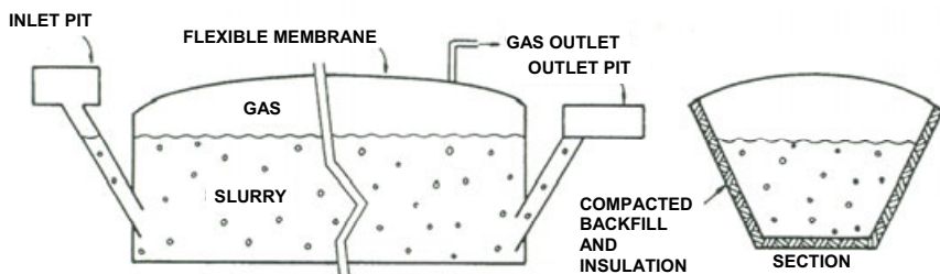
Figure 4.10 Plug-flow digester
