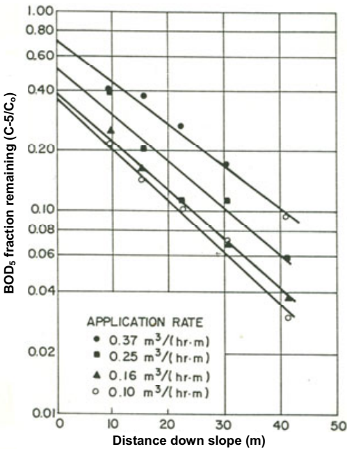
Figure 8.9 BOD 5 fraction remaining versus distance down-slope; application rate study with screened raw wastewater (Smith and Schroeder 1985)
