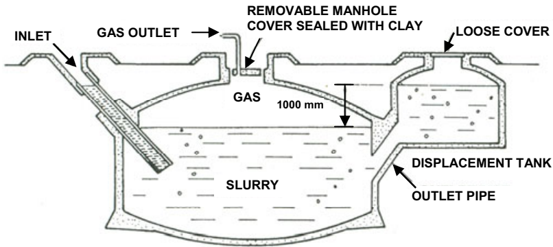
Figure 4.5 Fixed-dome digester
