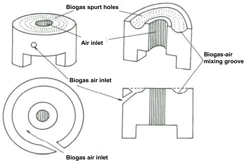
a) Earthen stove with mixing groove
