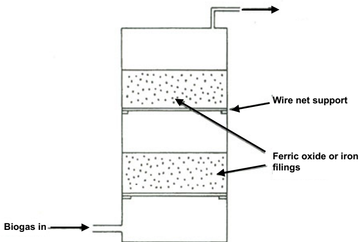
Figure 4.21 Model of dry gas scrubber for H_2S removal
