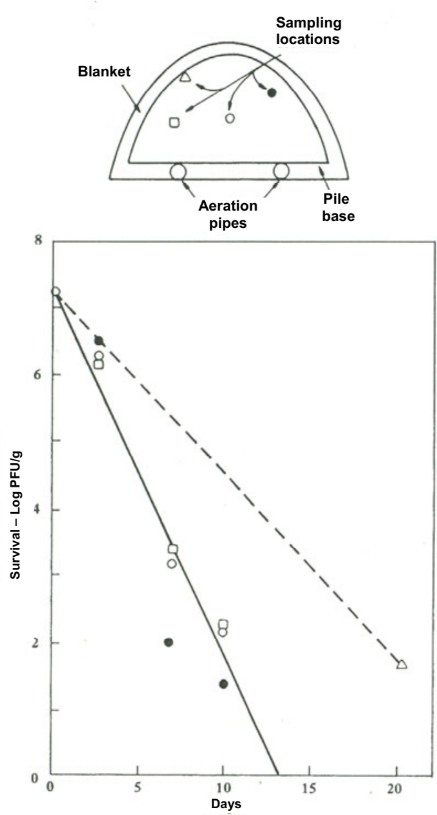
Figure 3.21 Destruction of F_2 bacteria virus during composting by the BARC system (U.S. EPA 1985)
