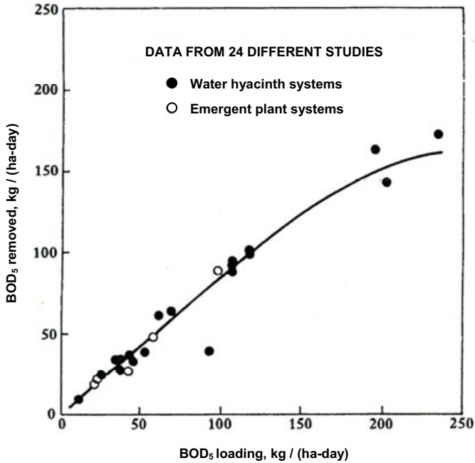
Figure 7.15 BOD removals as a function of BOD loading in aquatic systems (after Stowell et al. 1981; reproduced by permission of the American Society of Civil engineers)
