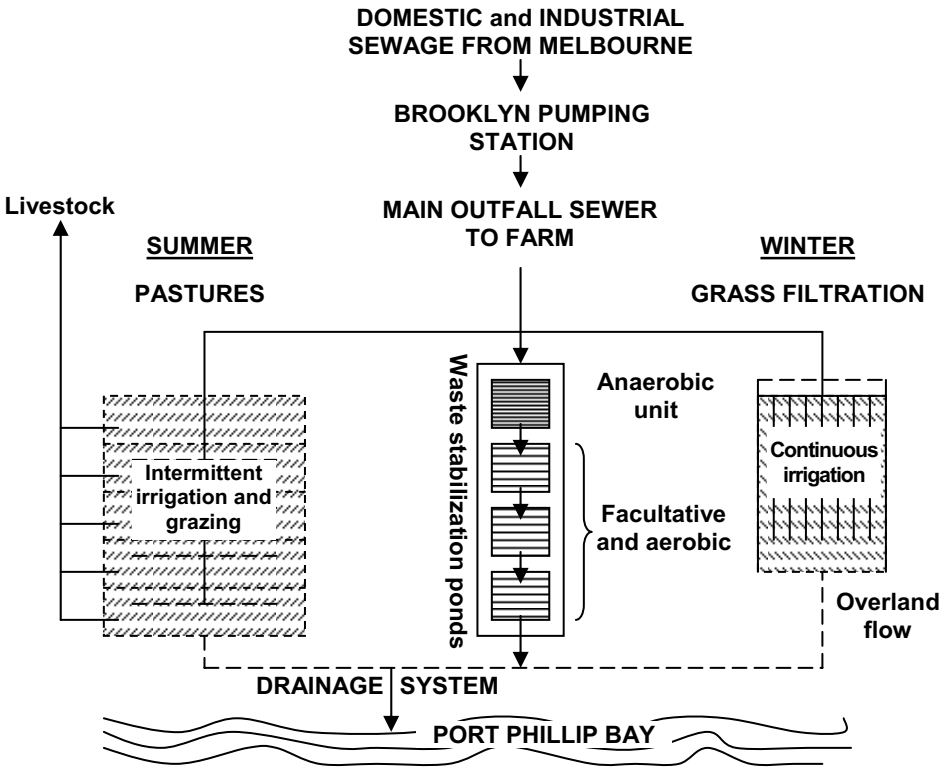
Figure 1.7 Sewage purification and waste recycling-Werribee Farm, Australia (Barnes 1978)
