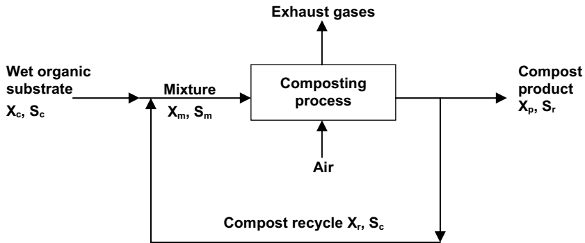
Figure 3.4 Schematic mass balance diagram for sludge composting showing inputs of compost feed and compost recycle, and compost product (adapted from Haung 1979; reproduced by permission of the Water Pollution Control Federation USA)
