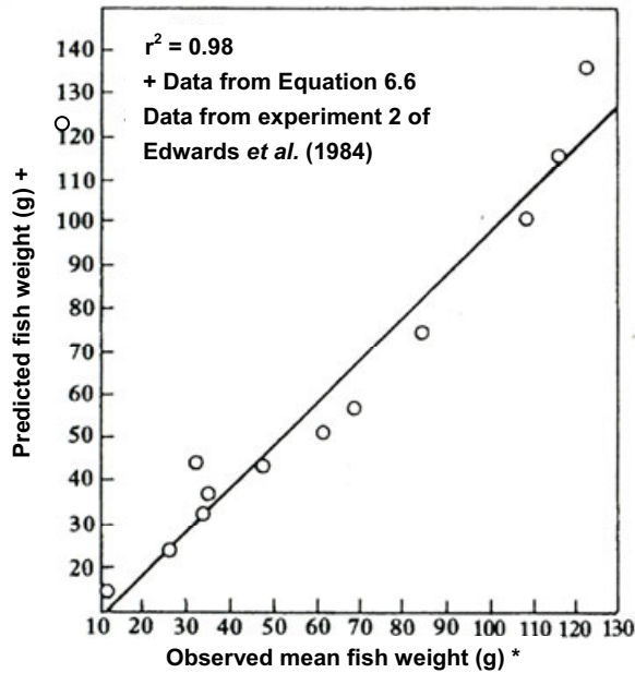
Figure 6.14 Observed versus predicted fish weight for septage-fed pond; SD = 1, 5; COD loadings = 150 kg/(ha-day)
