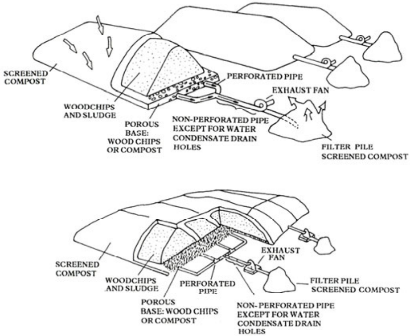
Figure 3.14 Configuration of aerated piles showing construction of pile and the arrangement of aeration pipe - the BARC system (Shuval et al. 1981; reproduced by permission of the World Bank)
