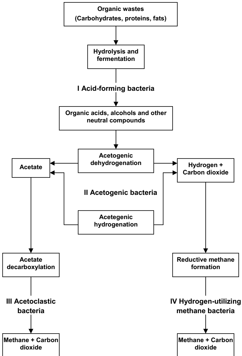
Figure 4.3 Biomethanation of organic wastes (Brown and Tata 1985)
