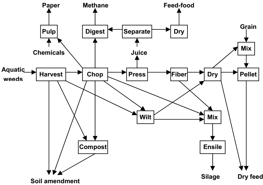
Figure 7.6 Different end products of harvested aquatic weeds (from Bagnell 1979; reproduced from the permission of the American Society of Agricultural (Engineers))
