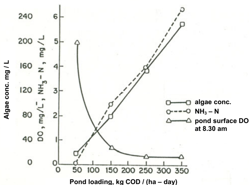
Figure 6.7 Effects of septage loadings on pond characteristics (no fish culture) from Polprasert et al. (1984); reproduced with permission of Pergamon Books Ltd
