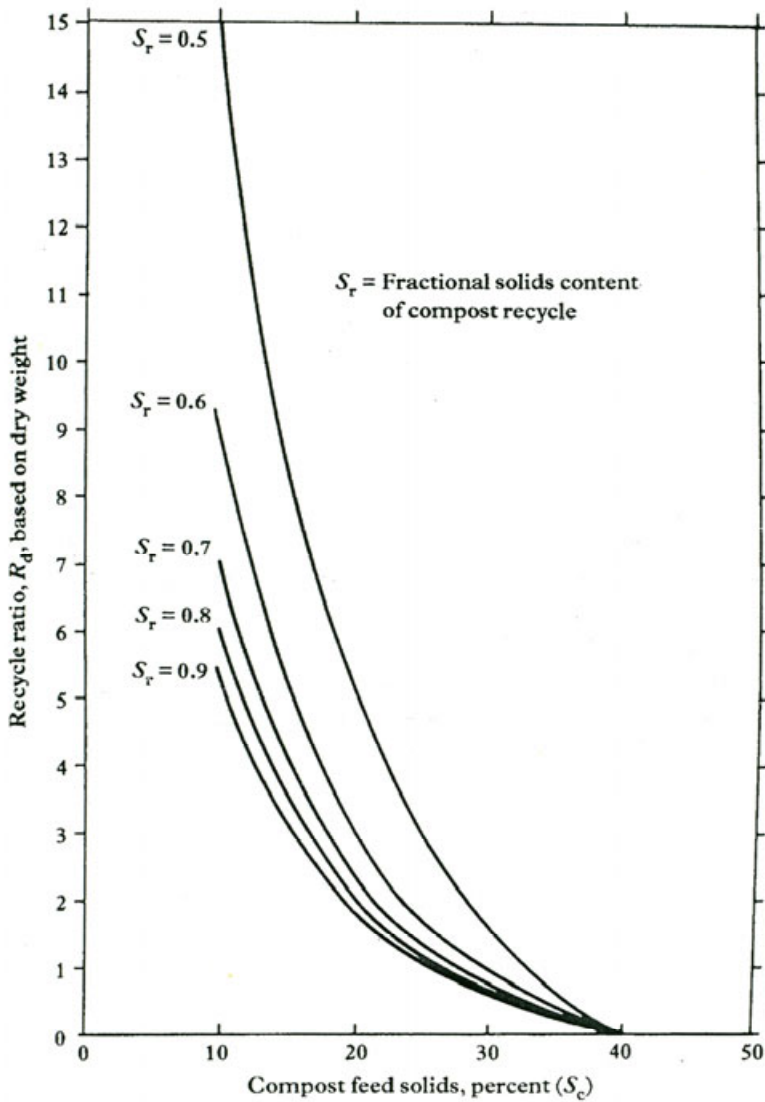
Figure 3.6 Effect of compost feed solids content on the dry-weight recycle ratio needed to achieve a 40 percent mixture solids content (Haug 1979; reproduced by permission of the Water Pollution Control Federation USA)
