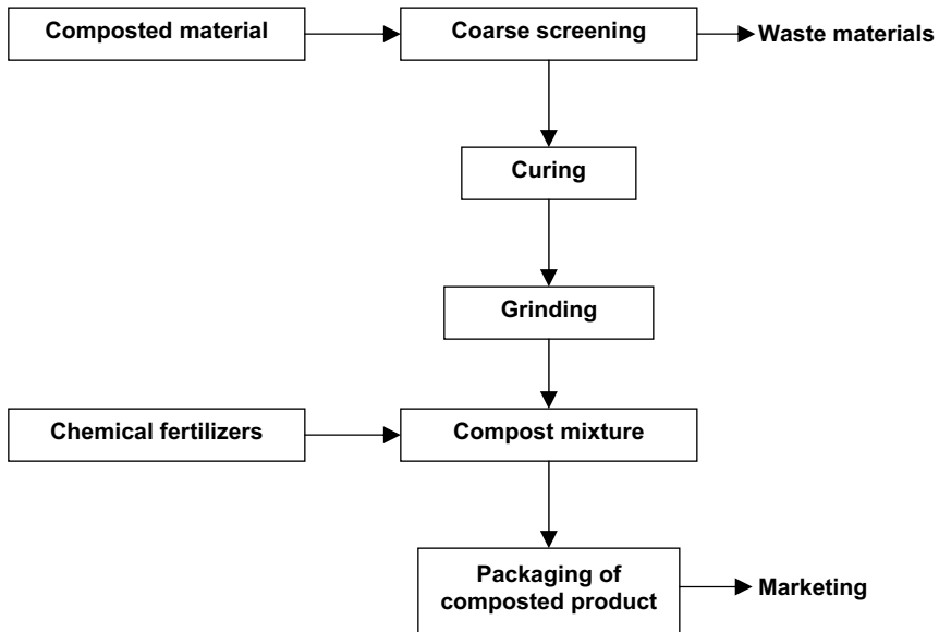
Figure 3.22 Flow chart of compost fertilizer production process
