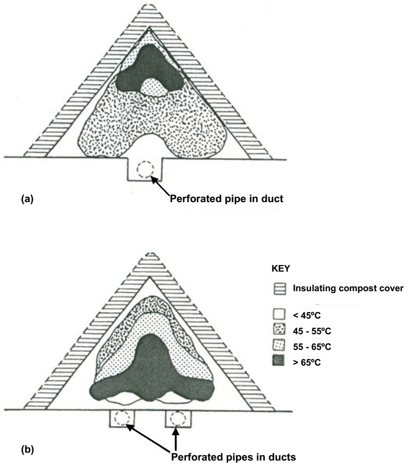
Figure 3.16 Typical temperature cross-section distributions in a pile with (a) positive pressure (blowing) aeration; and (b) negative pressure (sucking) aeration (from Stentiford et al. 1985; by permission of the Institute of Water Pollution Control, U.K.)
