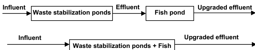
Figure 6.1 Layouts to upgrade waste stabilization pond (WSP) effluents using fish
