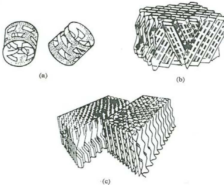
Figure 4.15 Packing media for anaerobic filters: (a) pall ring; (b) crossflow media; (c) tubular media
