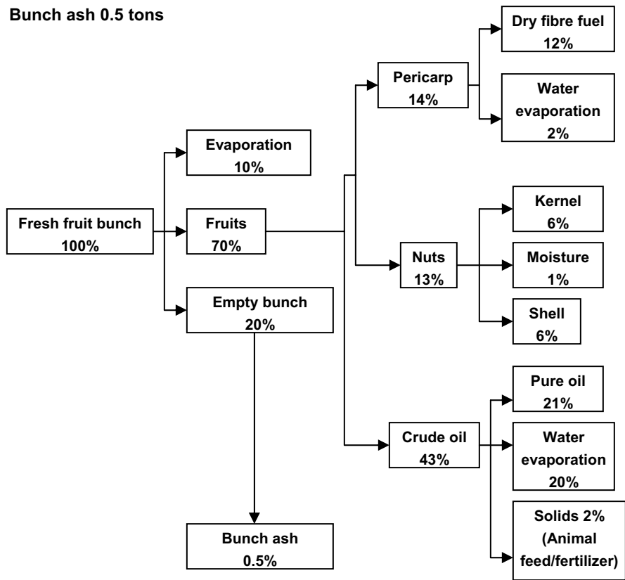
Figure 2.5 Product mass balance of a typical palm oil mill (Muttamara et al. 1987)
