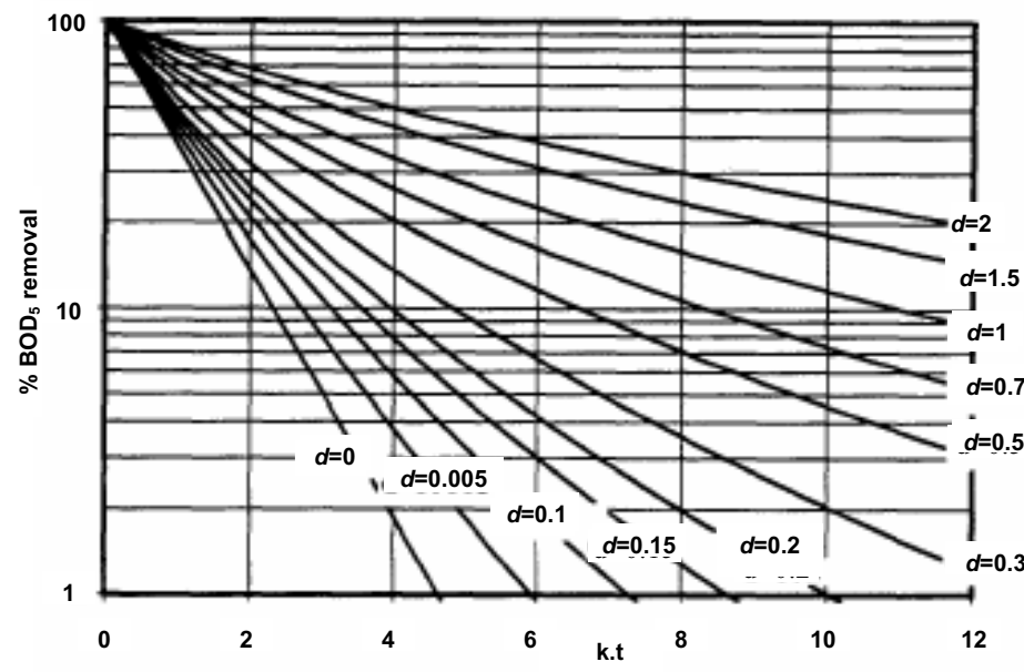
Figure 7.14 Design chart for BOD 5 removal in water hyacinth ponds (Polprasert et al. 1998)
