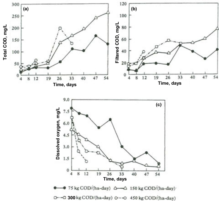
(a) Variation of total COD (b) Variation of filtered COD (c) Fluctuation of dissolved oxygen (DO) at dawn
