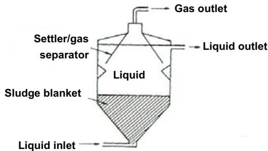
Figure 4.16 Upflow anaerobic sludge blanket digester
