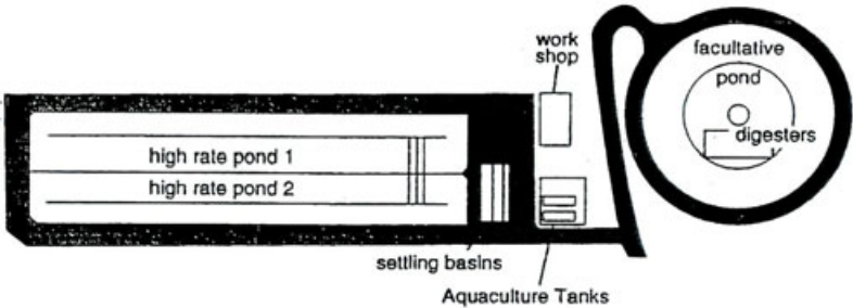
Figure 5.8 Advance integrated wastewater ponding system (Pilot plant at the University of California, Berkeley, Richmond Field Station, USA)
