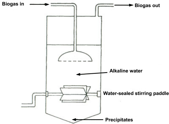
Figure 4.20 Model of \text{CO}_2 and \text{H}_2\text{S} scrubber in alkaline water
