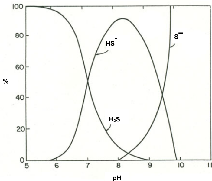
Figure 6.12 Effect of pH on hydrogen sulfide-sulfide equilibrium (after Sawyer et al. 2003; reproduced by permission of McGraw- Hill Book Company)
