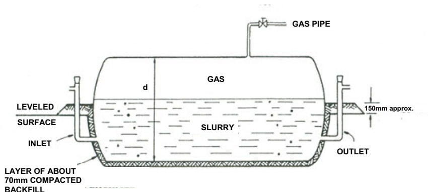
Figure 4.11 Bag digester
