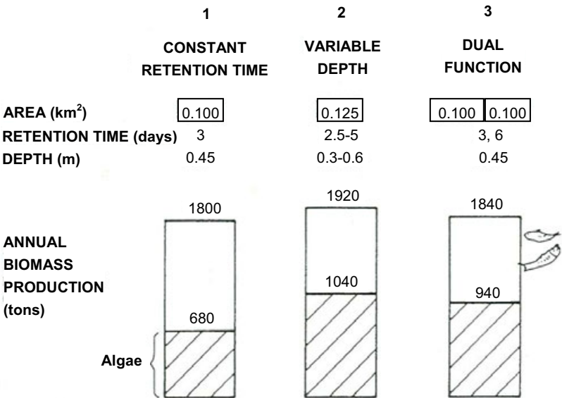
Figure 5.7. Three modes of HRAP operation.
