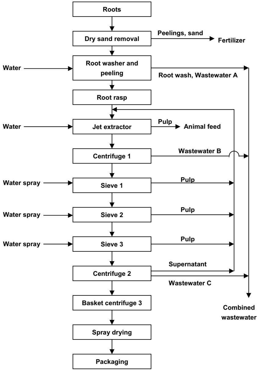
Figure 2.2 First-grade tapioca processing (Thanh 1984)
