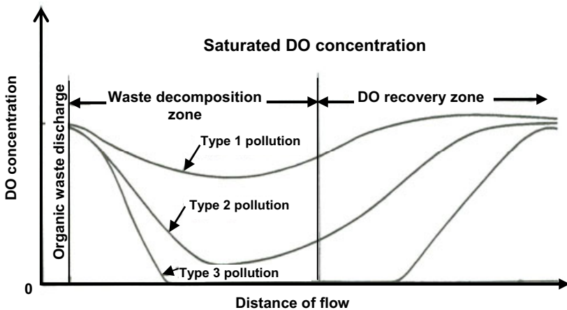
Figure 1.3 DO sag profile in polluted stream
