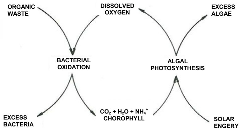
Figure 5.4 The cycle of oxygen and algal production in sewage treatment by photosynthesis (from Oswald and Gotaas 1955; reproduced by permission of the American Society of Civil Engineers)
