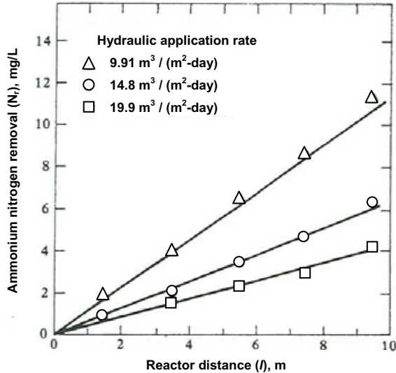
Figure 7.17 Ammonium nitrogen removal ( N_r ) as a function of reactor distance for three hydraulic application rates (after Weber and Tchobanglous 1986; reproduced by the permission of the Water Pollution Control Federation, USA)
