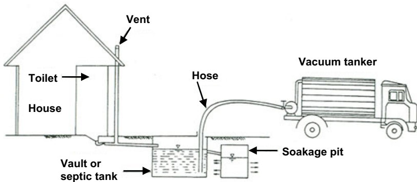
Figure 2.1 Vacuum tanker removing septage
