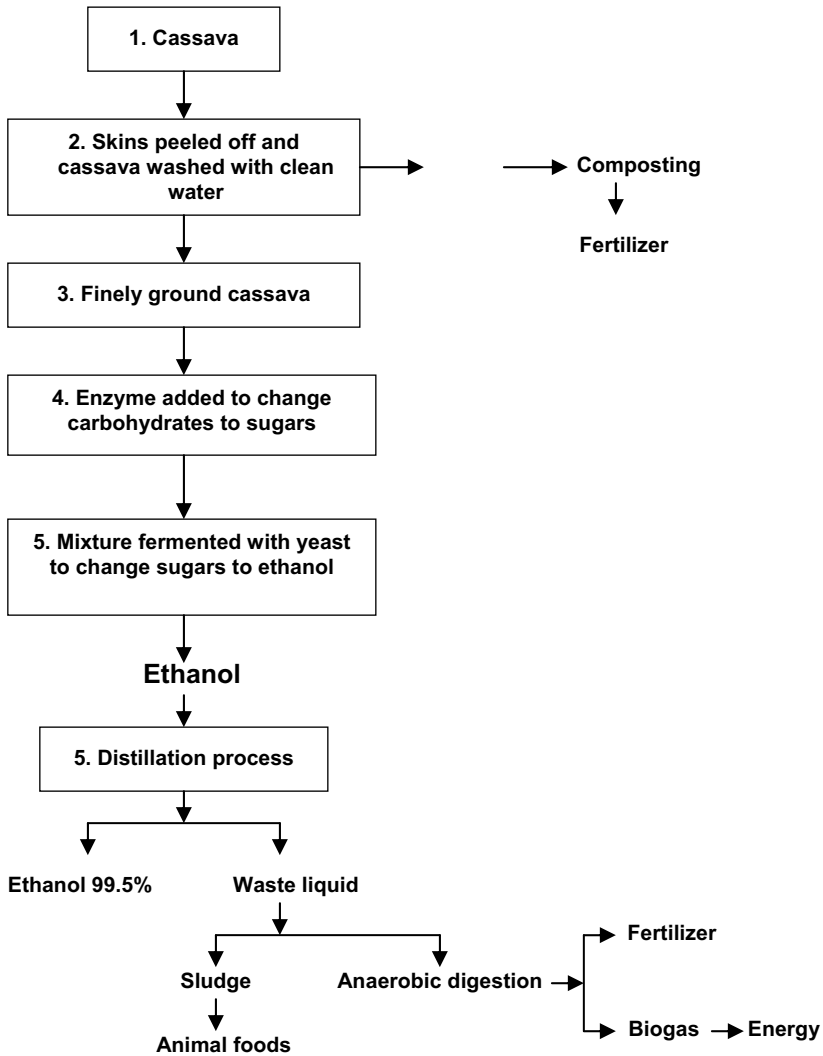
Figure 4.24 Ethanol production from cassava
