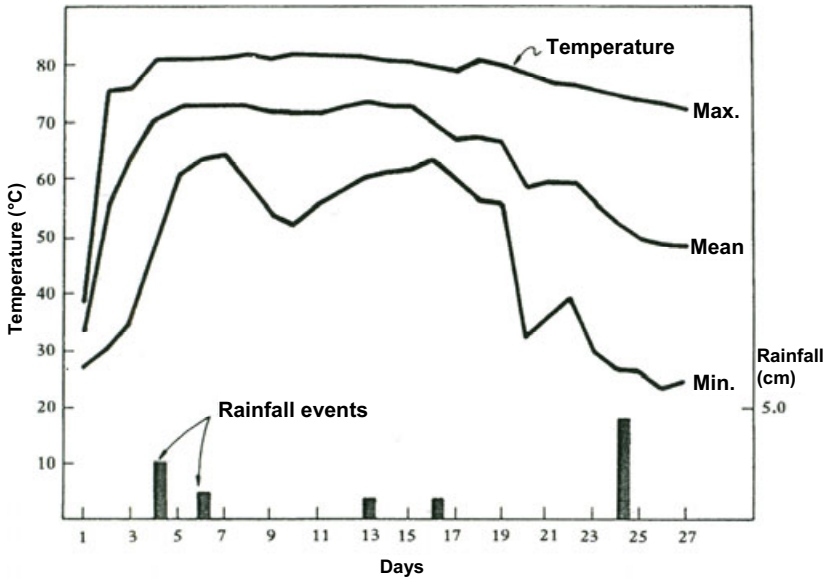
Figure 3.15 Temperature during sludge composting by the BARC system (Shuval et al. 1981)
