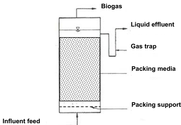
Figure 4.14 Up-flow anaerobic filter
