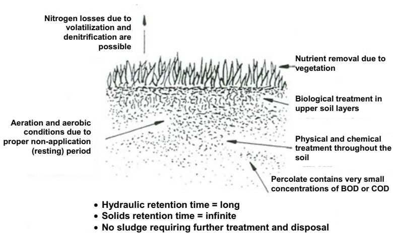
Figure 8.6 Waste management relationships that occur with land treatment (from Loehr and Overcash 1985; reproduced by the permission of the American Society of Civil Engineers)
