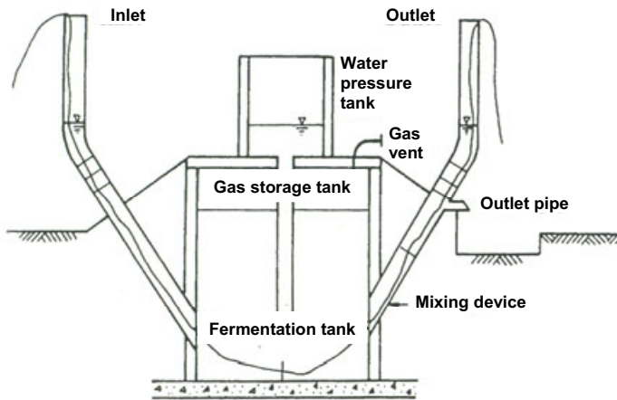
Figure 4.7 Low-cost biogas digester (note a unique mixing device)
