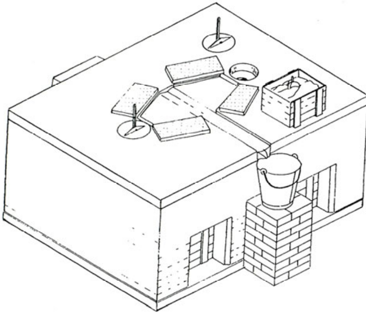
Figure 3.10 The Vietnamese composting toilet (Rybczynski et al. 1978; reproduced by permission of the International Development Research Centre, Canada)
