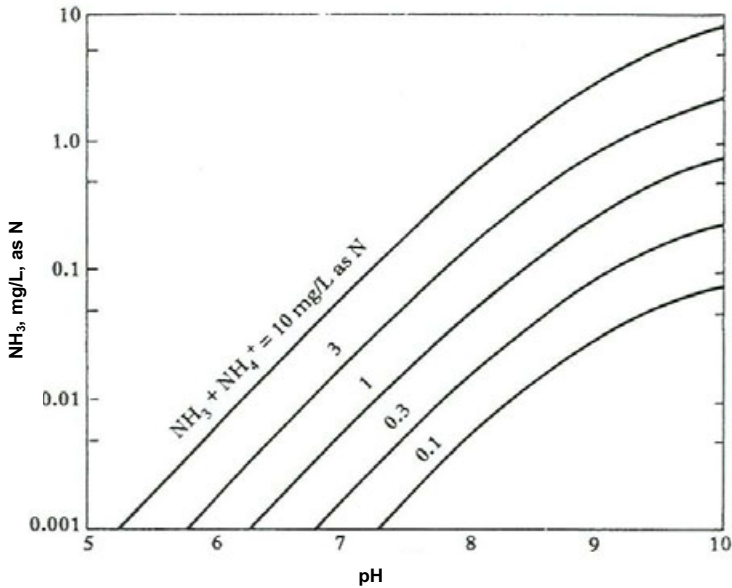
Figure 6.9 Effects of pH and ammonia nitrogen concentration ( \text{NH}_3 + \text{NH}_4^+ ) on the concentration of free ammonia in water (Sawyer et al. 2003; reproduced by permission of McGraw-Hill Book Company)
