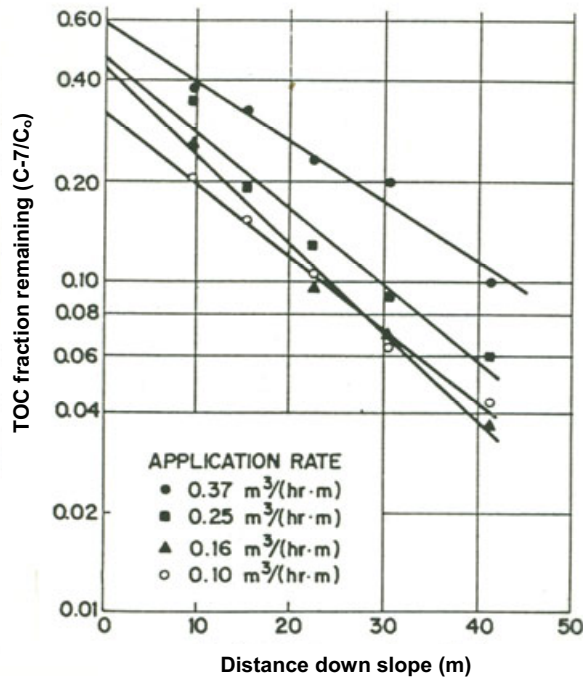
Figure 8.12 TOC fraction remaining versus distance down-slope; application rate study with primary effluent (from Smith and Schroeder 1985; reproduced by permission of the Water Pollution Control Federation, USA)
