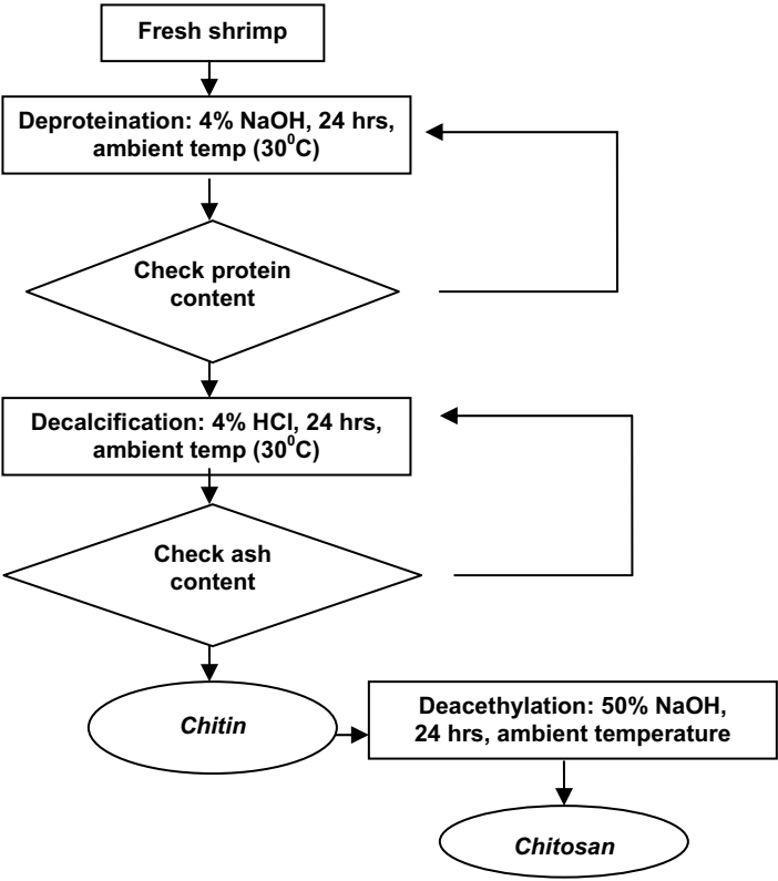
Figure 6.17 Production of Chitin and Chitosan
