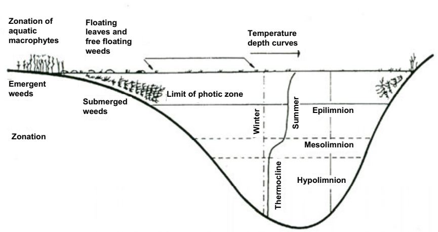
Figure 7.4 A diagrammatic representation of a lake showing zonation of aquatic weeds, the photic zone, and thermal stratification (adapted from Mitchell 1974; ©UNESCO 1974; reproduced by permission of UNESCO)
