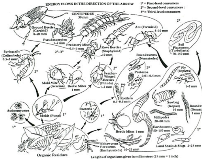
Figure 3.3 Food web of the compost pile (Dindal 1978; reproduced by permission of the JG Press)
