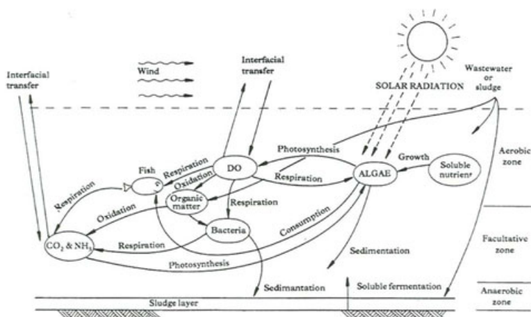
Figure 6.5 A simplified view of septage-fed fish pond dynamics (adapted from Bhattarai 1985)
