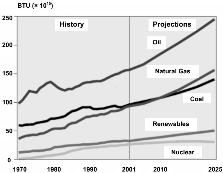
Figure 1.2 Energy consumption increases and changes in use pattern with human advances in science and technology (Energy Information Administration 2004)
