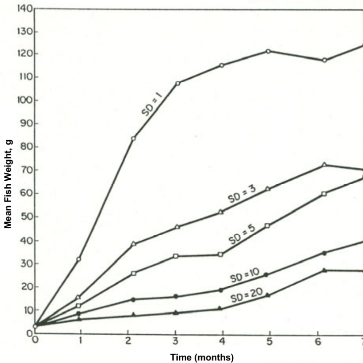
Figure 6.10 Mean individual fish weight (g) at monthly intervals in the septage-fed fish pond system. Each point is a mean of three ponds. Organic loading = 150 kg COD/ (ha-day). Stocking densities (SD) in number of fish/m 2 (Edwards et al. 1984)
