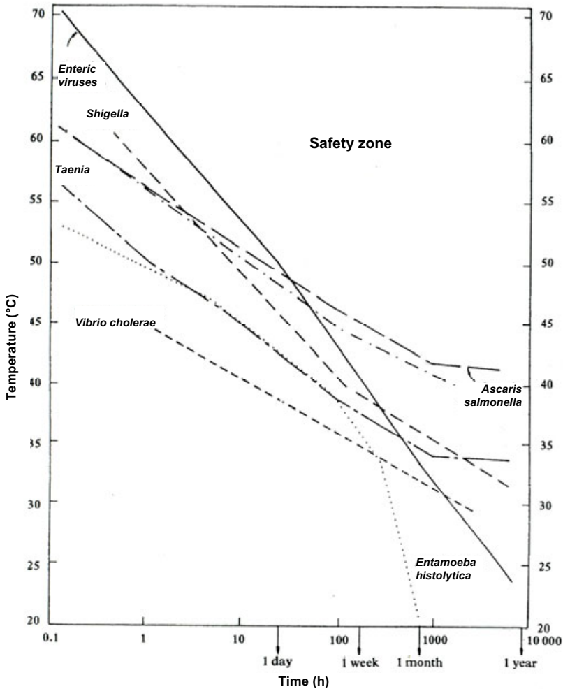
Figure 3.1 Influent of time and temperature on selected pathogens in night soil and sludge (Feachem et al. 1983; reproduced by permission of the World Bank). Note: The time represents conservative upper boundaries for pathogen death that is, estimates of time-temperature combinations required for pathogen inactivation. A treatment process with time-temperature effect falling within the “safety zone” should be lethal to all excreted pathogens (with the possible exception of hepatitis A virus – not included in the enteric viruses in the figure – at short retention time). Indicated time-temperature requirements are at least: 1 h at \geq 62^{\circ}\text{C} , 1 day at \geq 50^{\circ}\text{C} and 1 week at \geq 46^{\circ}\text{C}
