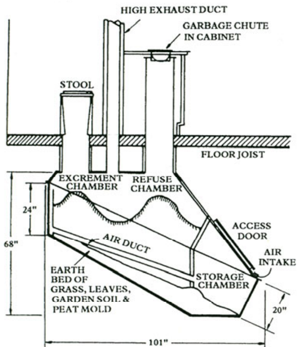
Figure 3.7 The Clivus Multrum (Rybczynski et al. 1978; reproduced by permission of the International Development Research Centre, Canada)
