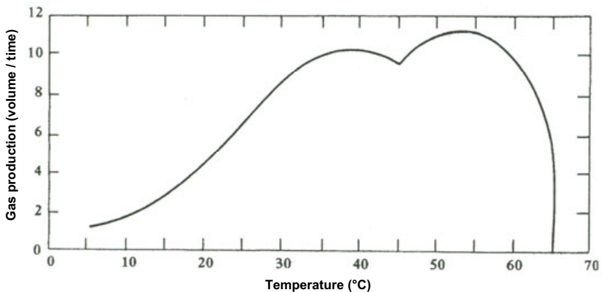
Figure 4.4 Effect of temperature on gas production (Price and Chermisinoff 1981)
