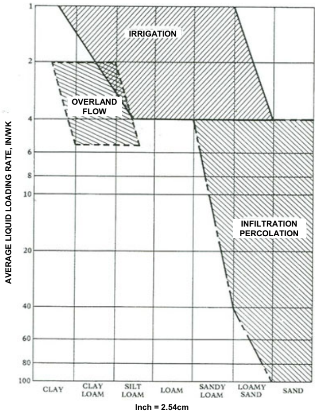
Figure 8.1 Soil type vs liquid loading rates for different load application approaches (U.S. EPA 1976)
