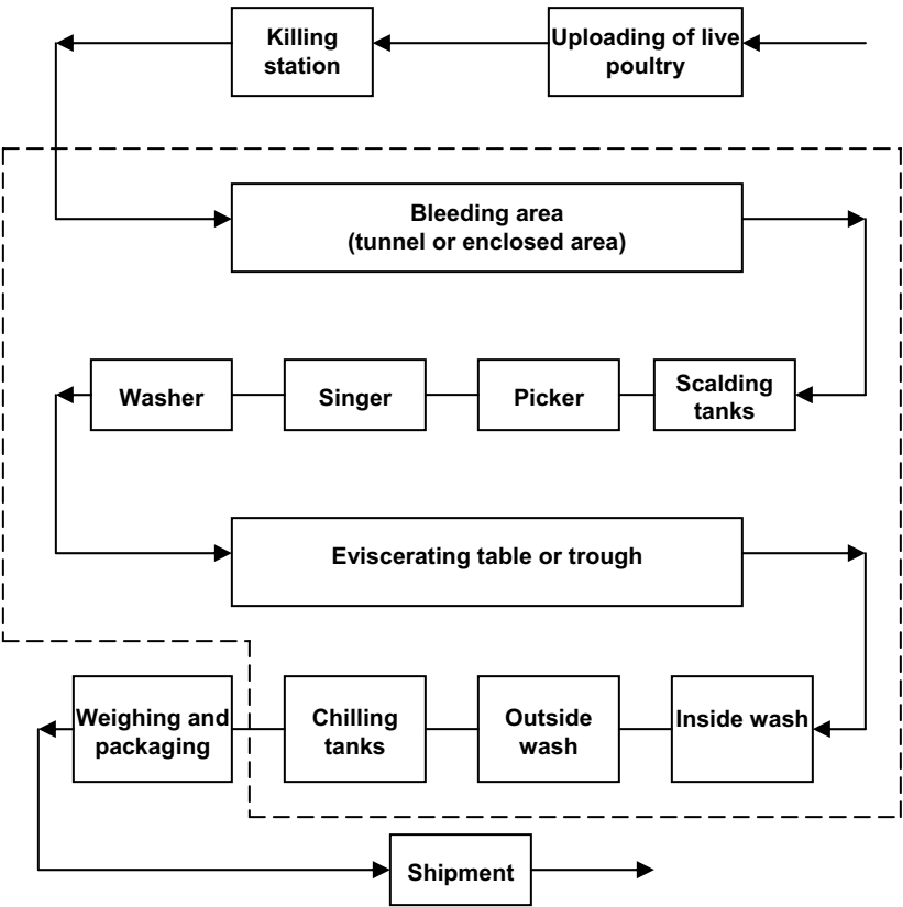
Figure 2.9 Major steps in poultry processing (Nemerow 1971) (© 1971, Addison Wesley Publishing Co., Reading, Mass)
