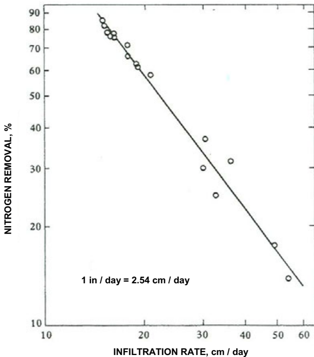
Figure 8.8 Effect of infiltration rate on nitrogen removal for rapid infiltration, Phoenix, Arizona (From Lance and Gerba 1977; reproduced by the permission of Pergamon Books Ltd)
