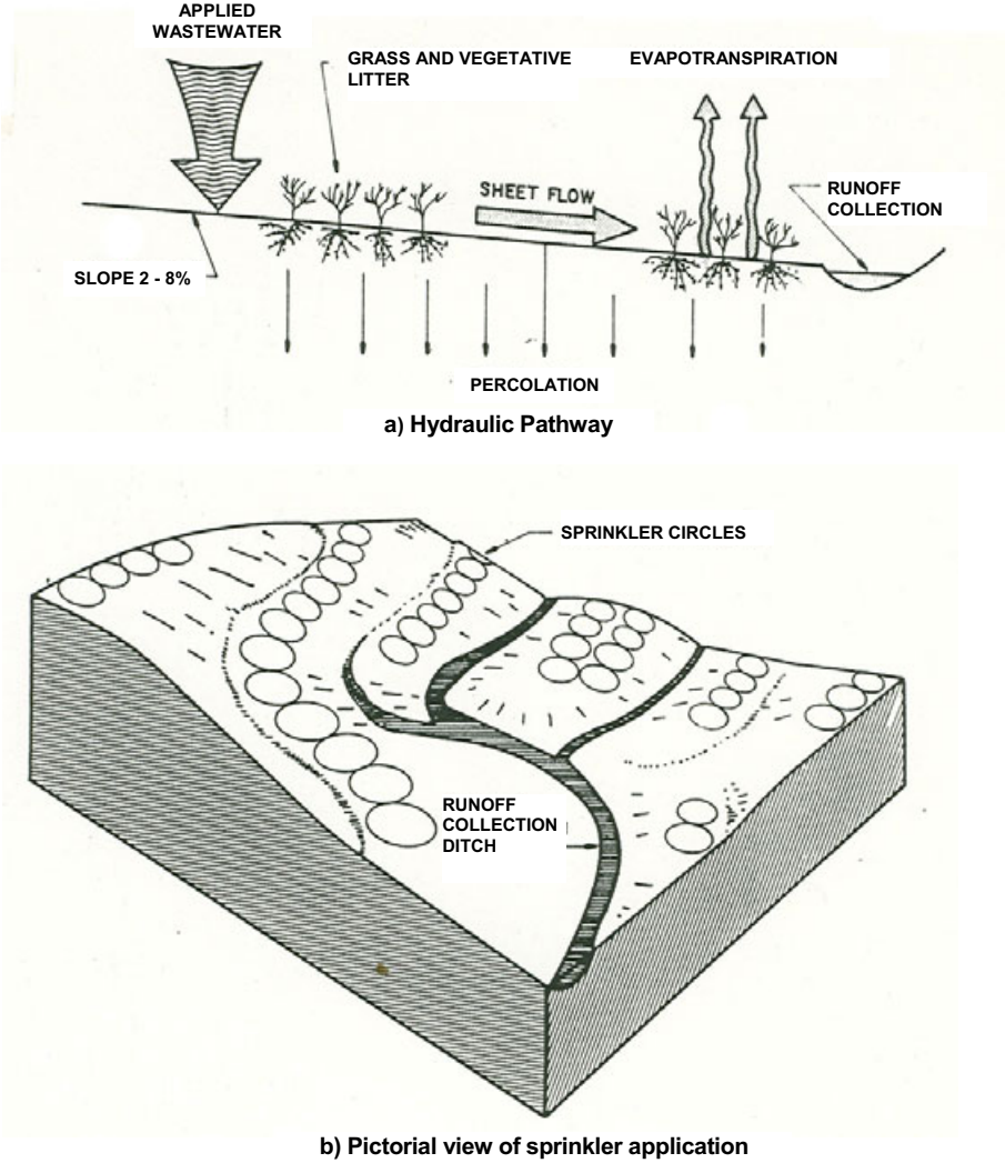
Figure 8.4 Overland flow (U.S.EPA 1981)
