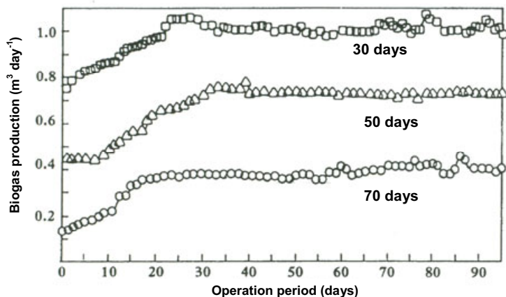
Figure 4.8 Mean daily biogas production at hydraulic retention times of 30, 50, and 70 days from pilot small-scale digesters. Each point is the mean of four digesters.
