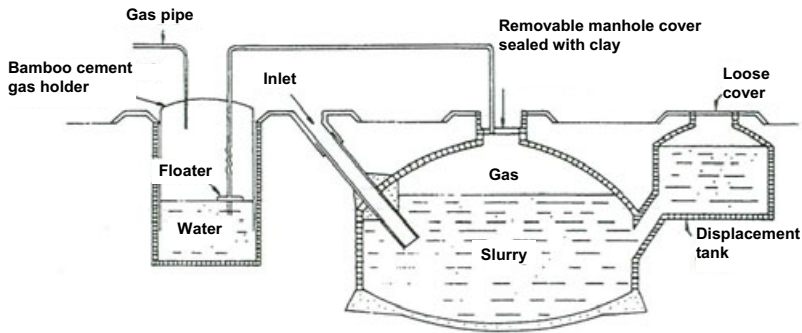
Figure 4.12 Fixed-dome digester with separate gas holder
