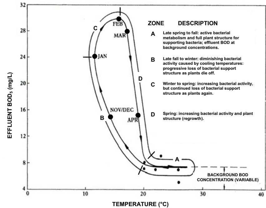
Figure 7.11 An example of the seasonality of effluent BOD 5 concentrations. Note: Compiled by Stowell et al. (1980), using data from Wolverton and McDonald (1976a). Reproduced by permission
