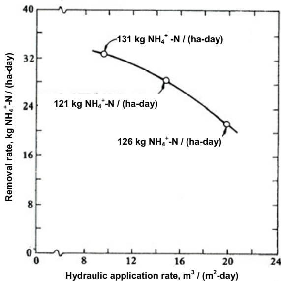
Figure 7.16 NH_4^{+}\text{-N} removal as a function of hydraulic application rate (corresponding loading rates for NH_4^{+}\text{-N} are as shown) (after Weber and Tchobanoglous 1985; reproduced by permission of the Water Pollution Control Federation, USA)
