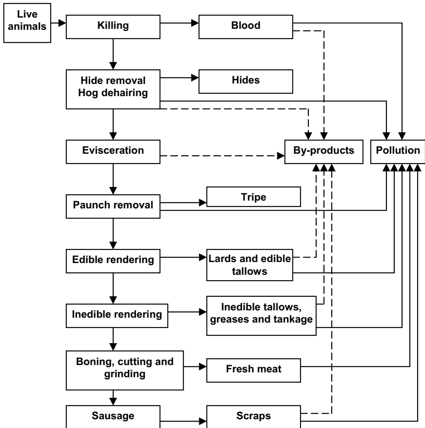
Figure 2.8 Fundamental processes in a slaughterhouse (Nemerow 1971) (© 1971, Addison-Wesley Publishing Co., Reading, Mass)
