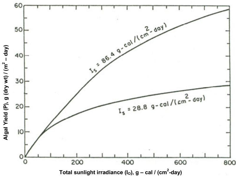
Figure 5.9 Algal yield ( P_a ) as a function of total solar irradiance ( I_0 ) according to Equation 5.5 (adapted from Goldman 1979b; reproduced by permission of Pergamon Books Ltd)
