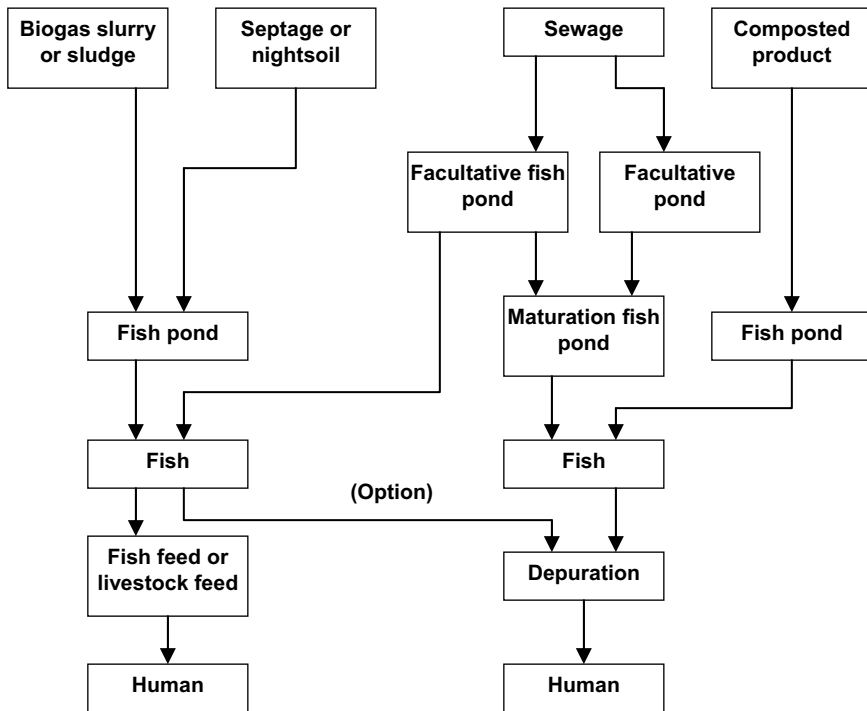
Figure 6.15 Some arrangements of waste-fed ponds
