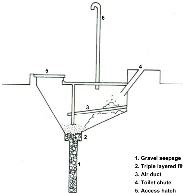
Figure 3.8 The Biopit composting toilet (Rybczynski et al. 1978; reproduced by permission of the International Development Research Centre, Canada)
