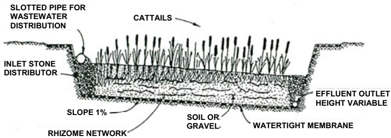
Figure 7.18 Typical cross-section of SF constructed wetlands (U.S. EPA 1988)
