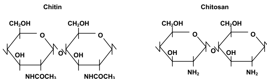
Figure 6.16 Chemical structures of chitin and chitosan
