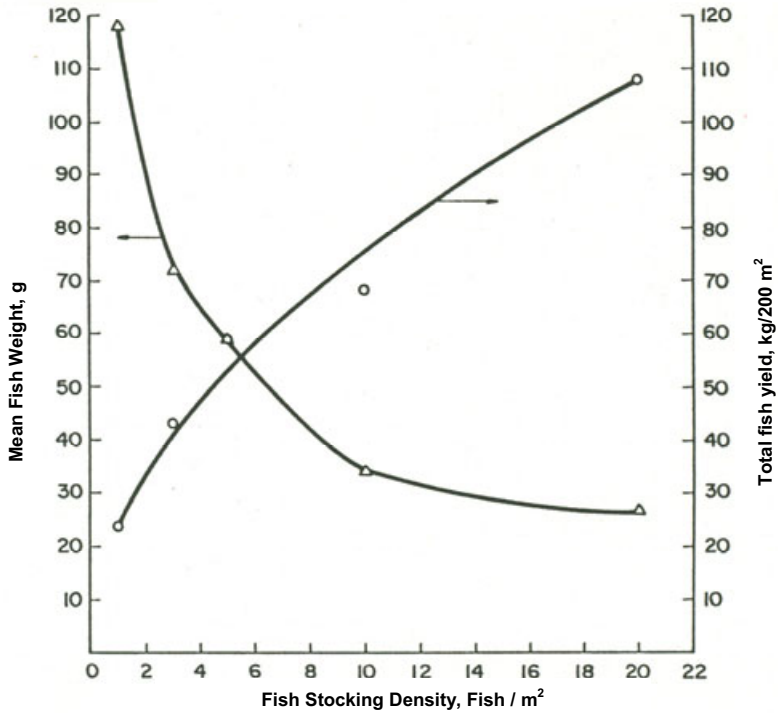
Figure 6.11 Effects of fish stocking density on mean fish weight and total fish yield after 6 months of pond operation. Data obtained from Figure 6.10 and assuming no fish mortality and no spawning
