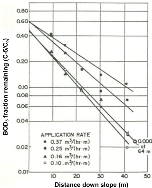
Figure 8.11 BOD 5 fraction remaining versus distance down-slope; application rate study with primary effluent (Smith and Schroeder 1985)
