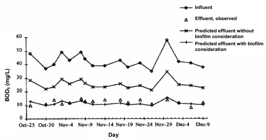
Figure 7.13 Predicted and observed effluent BOD 5 concentration of the WHP (Polprasert and Khatiwada 1998)
