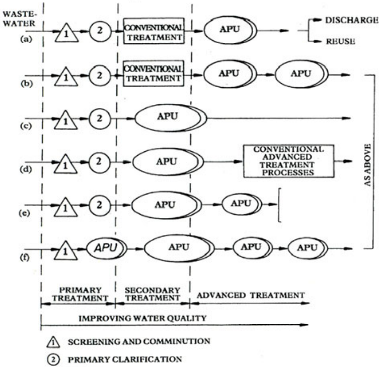
Figure 7.12 Conceptual uses of APUs (aquatic processing units) for the treatment of wastewater (Tchobanoglous et al. 1979)
