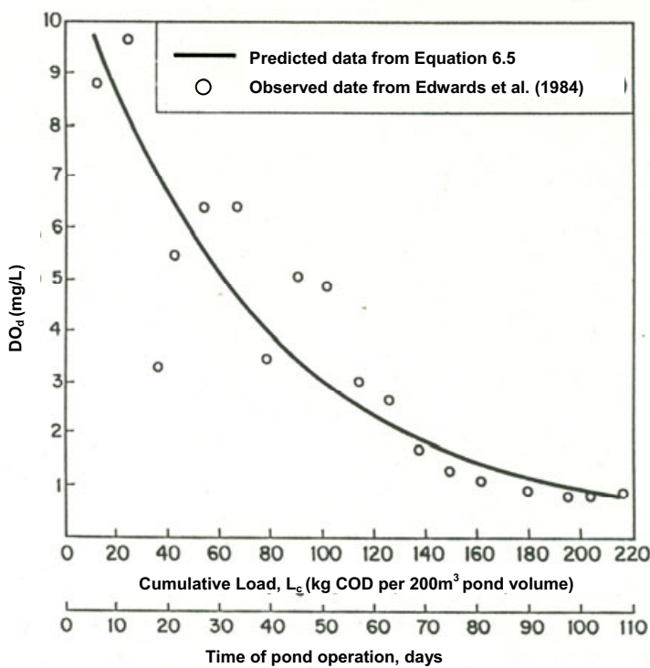
Figure 6.13 Cumulative load versus DO d for 100 kg COD/(ha-day) loaded septage ponds
