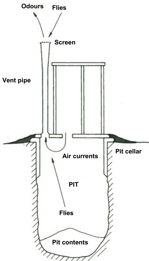
Figure 3.9 Schematic diagram of a ventilated improved pit latrine (Morgan and Mara 1982; reproduced by permission of the World Bank)
