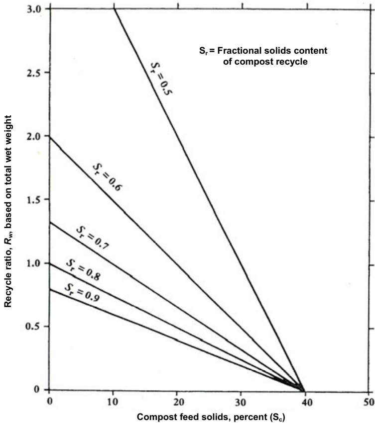
Figure 3.5 Effect of compost feed solids content on the wet weight recycle ratio needed to achieve a 40% mixture solids content (Haug 1979; reproduced by permission of the Water Pollution Control Federation USA)
