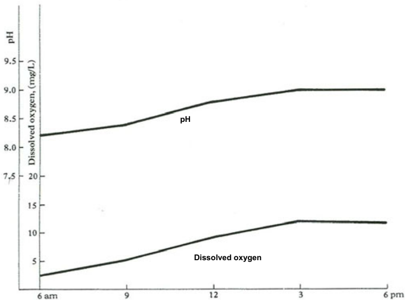
Figure 6.6 Semi-diurnal studies of the septage-fed pond system. Dissolved oxygen and pH were measured at 3 hr interval from 6 a.m. to 6 p.m. on four occasions. Mean of 15 septage fed ponds with fish stocking densities of 3, 6, 9, 12, and 15 /m 2 in triplicate (Polprasert et al. 1985)
