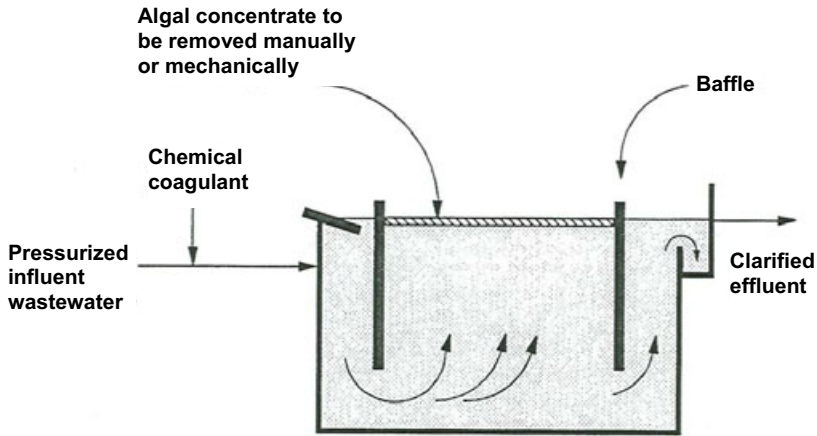
Figure 5.12 Schematic of a dissolved air flotation unit
