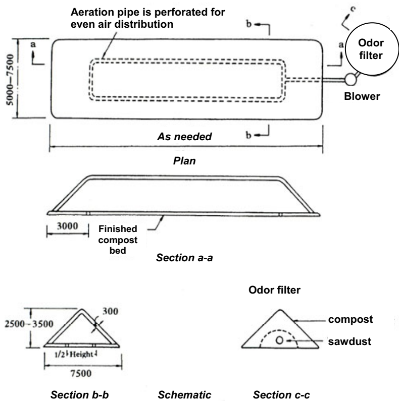
Figure 3.13 Schematic diagram of an aerated pile indicating location of aeration pipe. Loop is perforated for air distribution system (units in millimetres) (Shuval et al. 1981; reproduced by permission of the World Bank)
