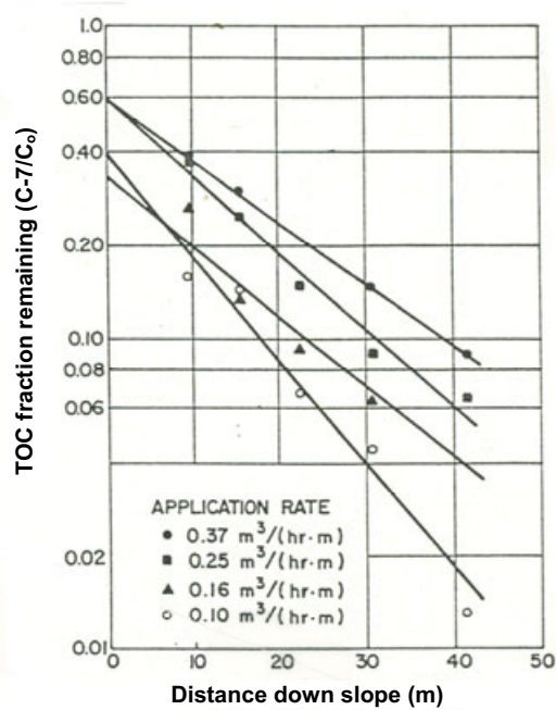
Figure 8.10 TOC fraction remaining versus distance down-slope; application rate study with screened raw wastewater (Smith and Schroeder 1985)
