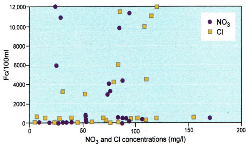
Figure C13 Lusaka waterwell fecal coliform (FC), nitrate ( \text{NO}_3 ) and chloride ( \text{Cl} ) data (high FC counts correspond to shallow private wells but deeper utility wells are not generally affected, although can have high nitrate levels).
