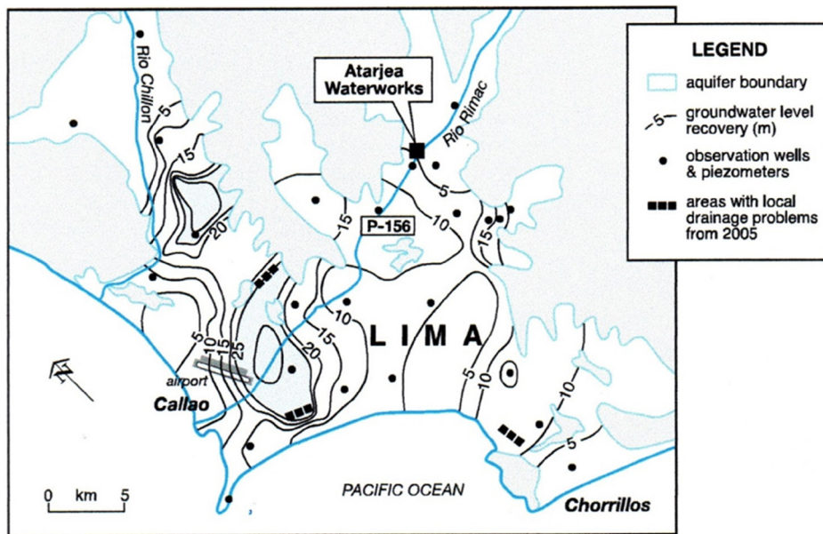
Figure C3 Distribution of Greater Lima aquifer system and its water table recovery during 1997–2003.
