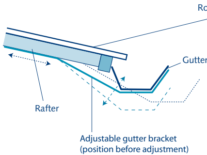
Figure 8.7a. Rafter mounting
