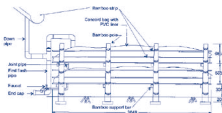
General Assembly Diagram
