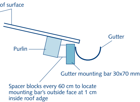
Figure 8.7b. Purlin mounting
