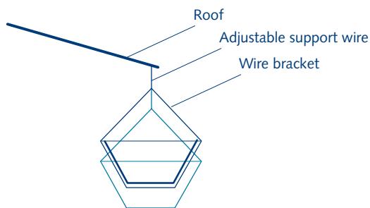
a. Usual suspended mounting method
