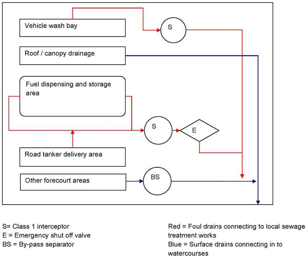
Figure 25: Typical site drainage plan for a refuelling facility (Environment Agency for England and Wales, the Northern Ireland Environment Agency and the Scottish Environment Protection Agency, 2011)
