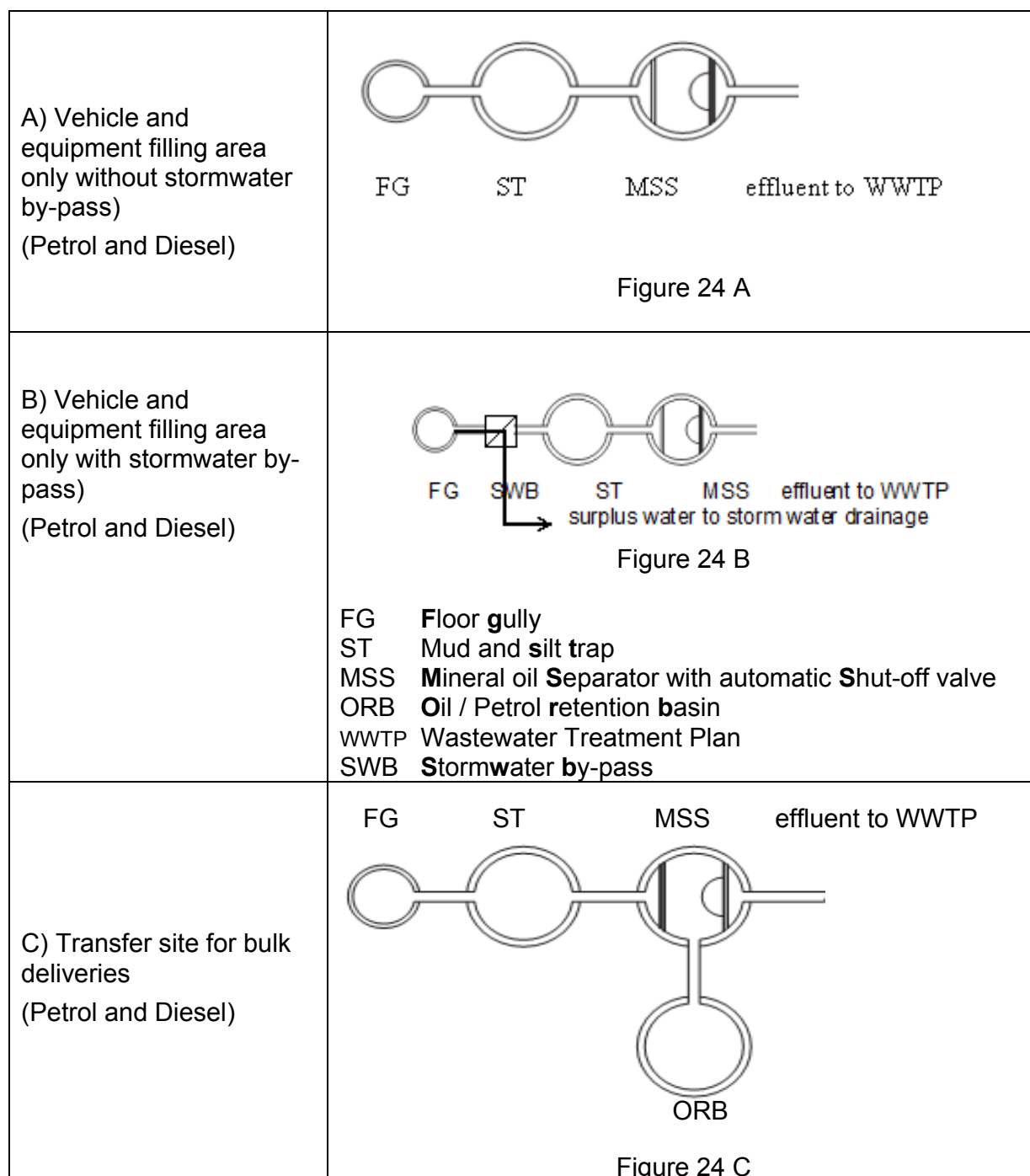
Figure 24: Design Principles for Drainage System of Gas Stations
