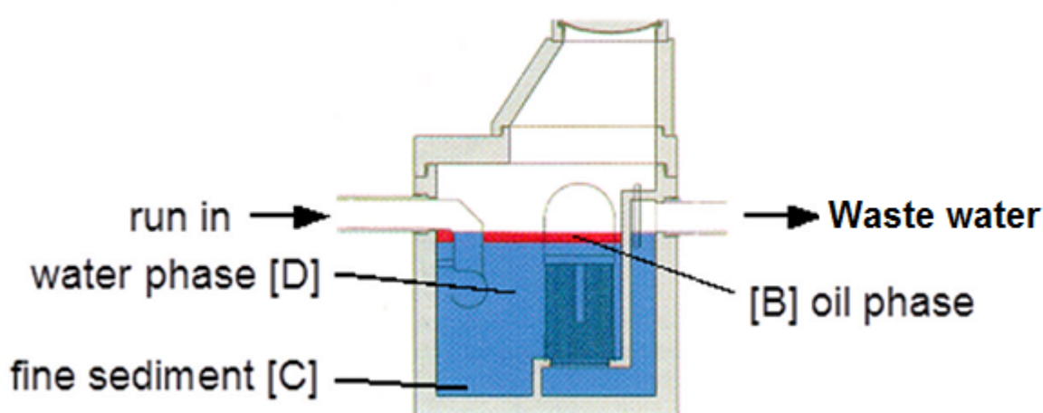
Figure 27: Coalescence separator
